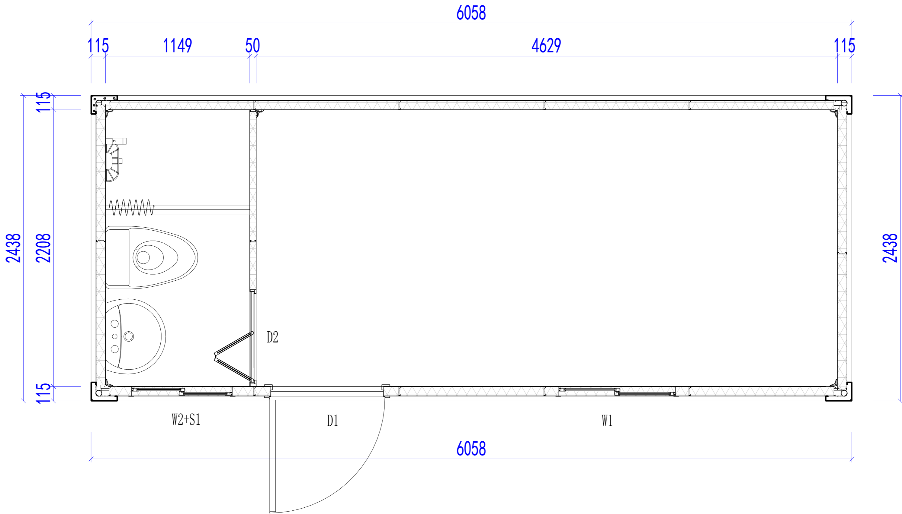
LAYOUT PLAN
