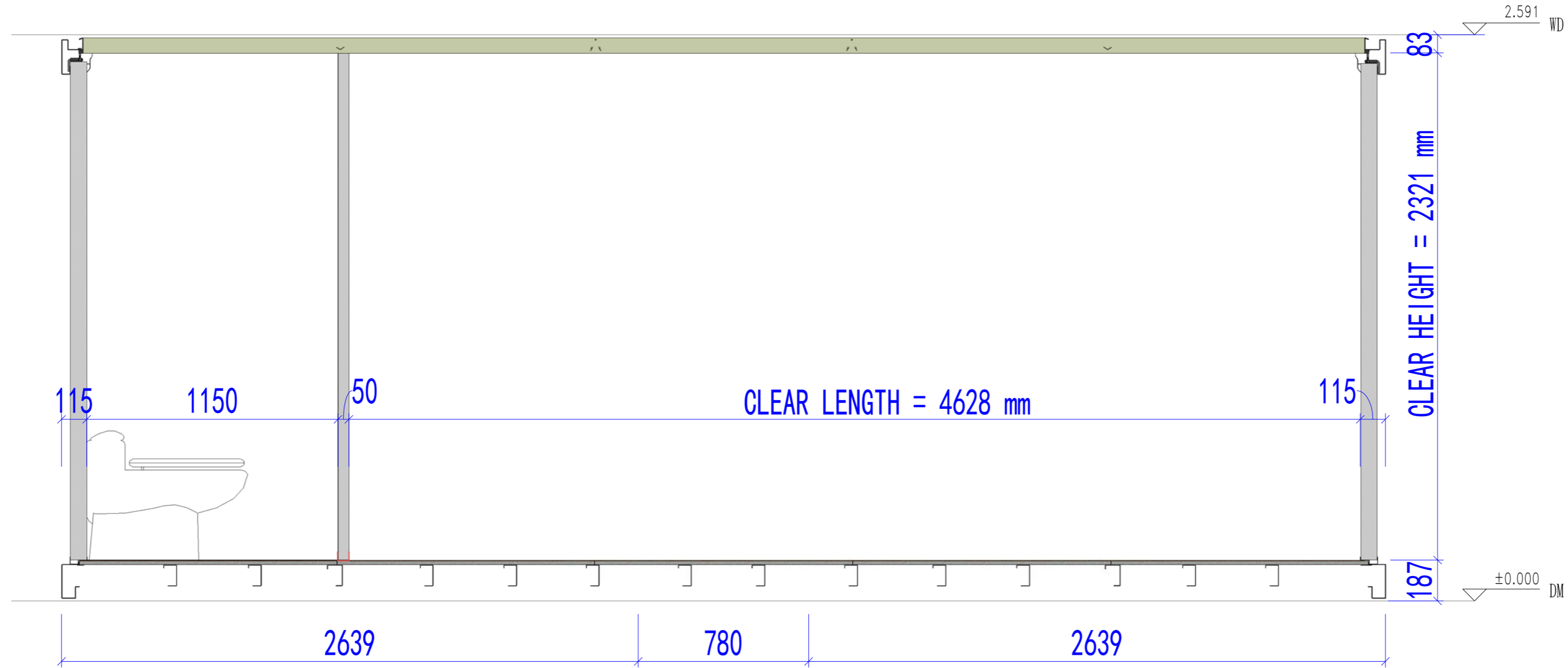
SECTION PLAN
